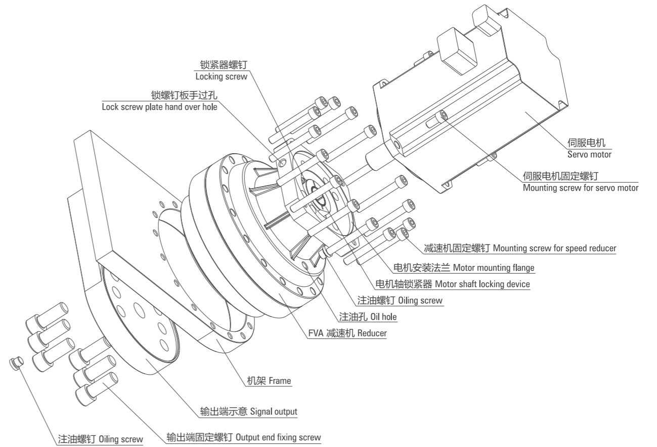
FVA系列减速机安装拆解示意图 FVA Series Mounting Schematic Diagram (Disassemble Diagram)
